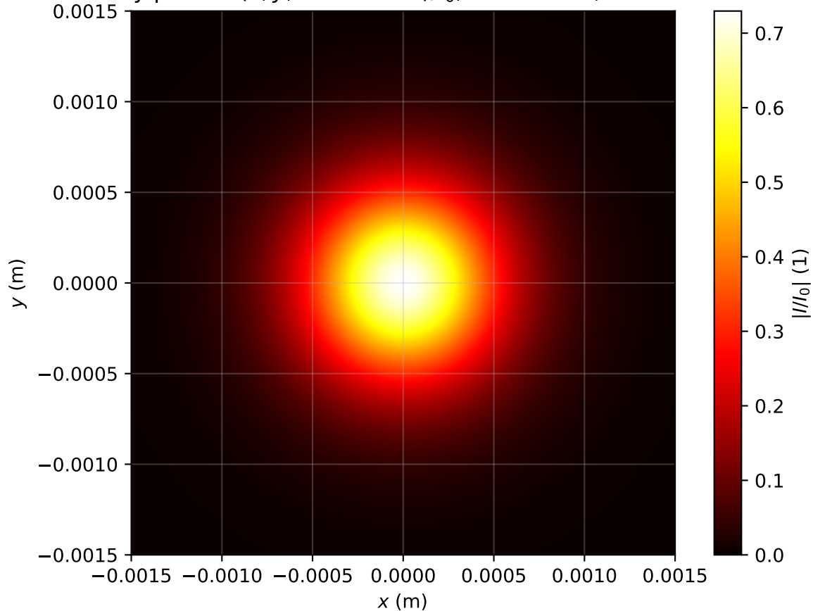
Intensity profile I(x, y, z = 2.786m)/I_0 , Pin=0.6Pcr, artificial time
